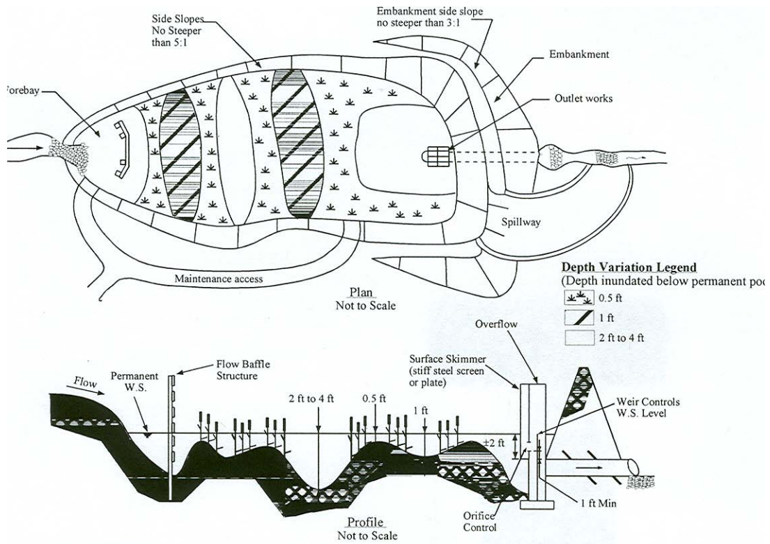
Figure PC-102A Typical Constructed Wetland Components (SUSMP, 2002)
