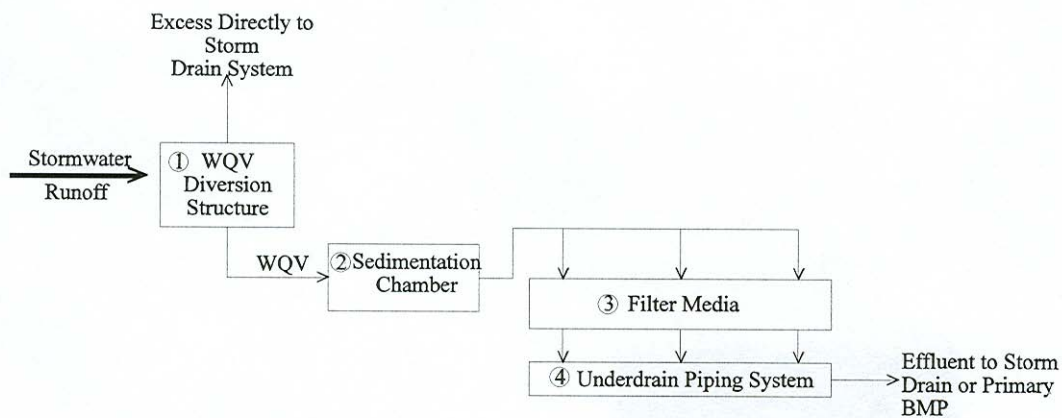
Figure PC-106A Typical Media Filtration Schematic (SUSMP, 2002)
