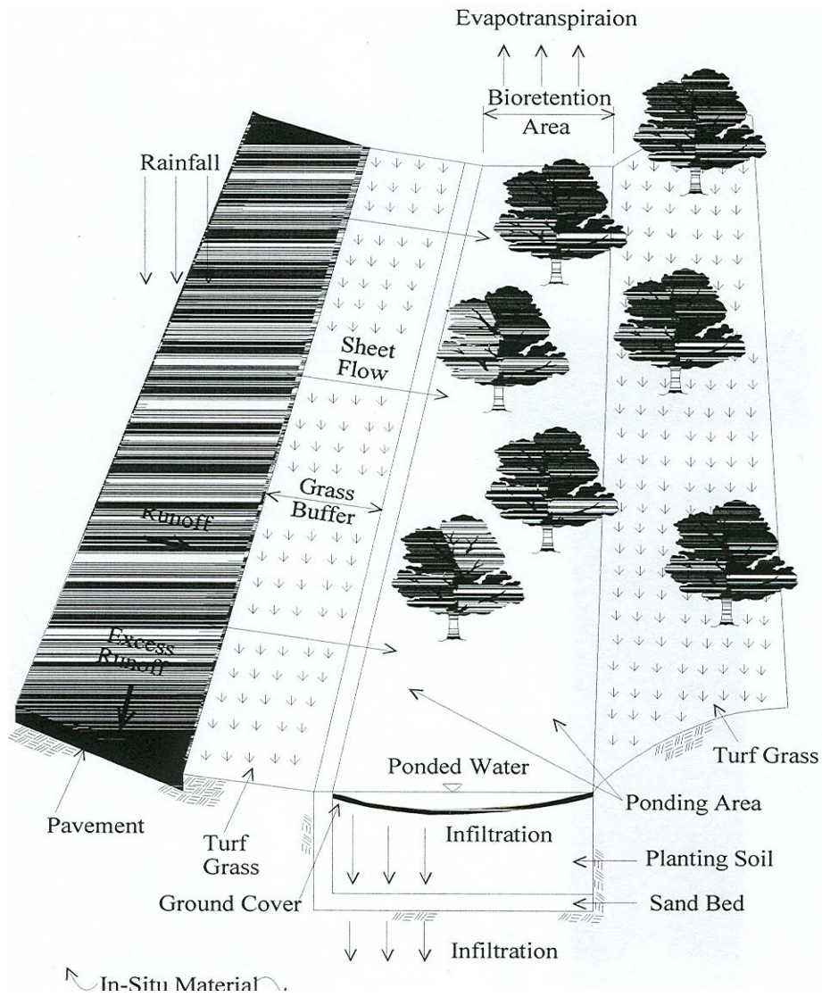
Figure PC-101A Schematic of Bioretention Area (SUSMP, 2002)
