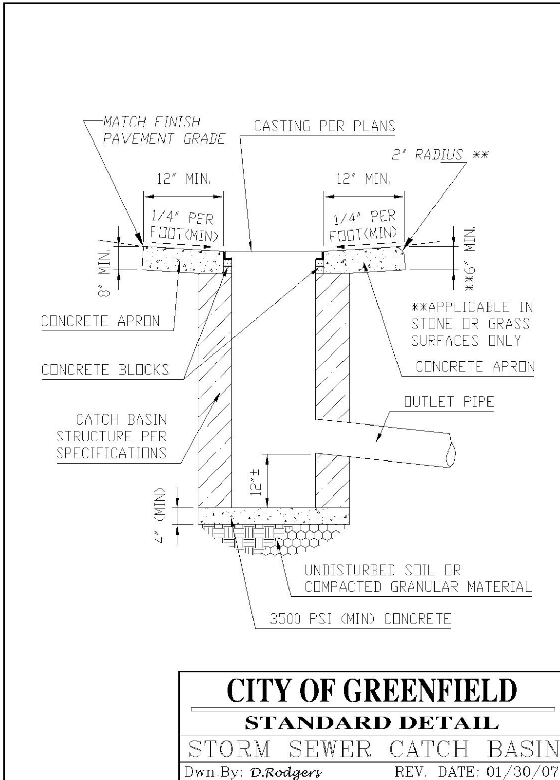
Figure 4-2 Standard Detail: Storm Sewer Catch Basin
