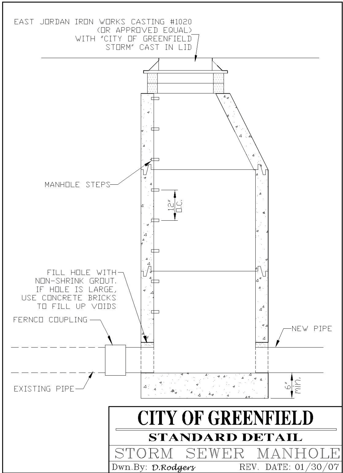
Figure 4-4 Standard Detail: Storm Sewer Manhole
