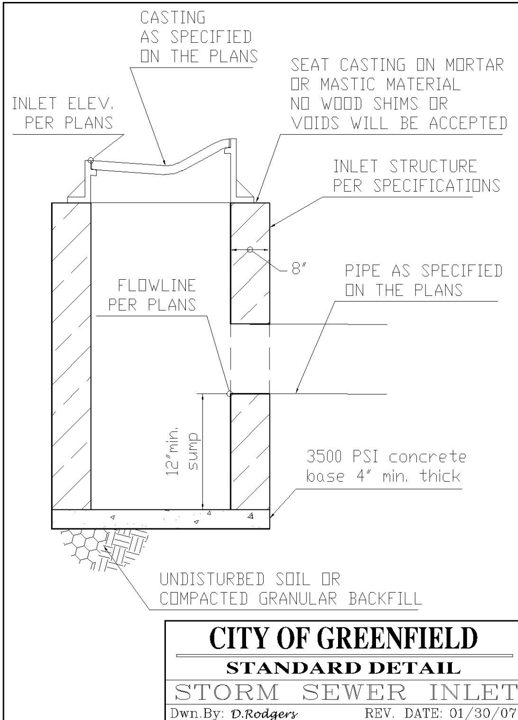
Figure 4-3 Standard Detail: Storm Sewer Inlet
