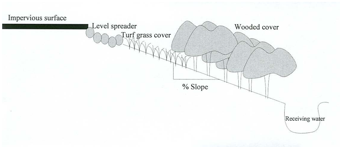
Figure PC-108A Typical Buffer Strip (SUSMP, 2002)
